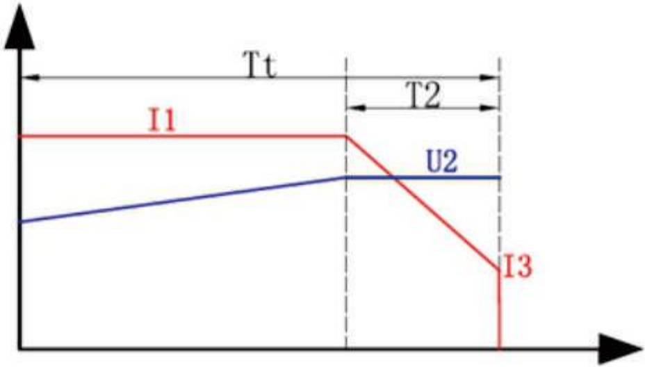
充电曲线 (IUa) Charging Curve (Iua)
